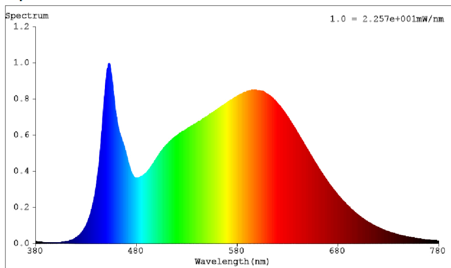
Spectral Distribution
